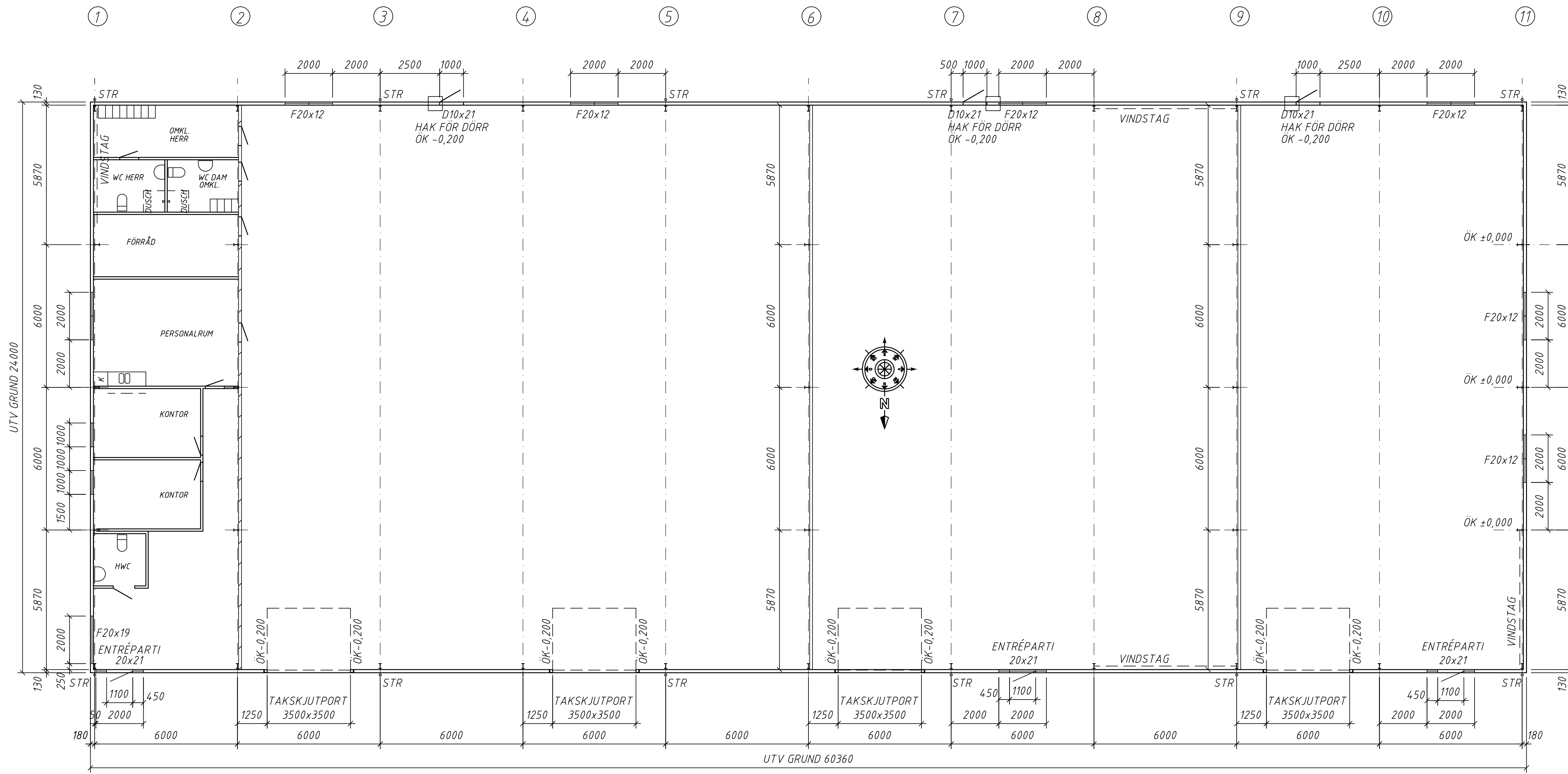
PLAN -1:100-
